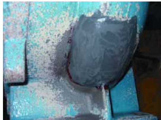
Repaired by coating with better durability than cast iron.
